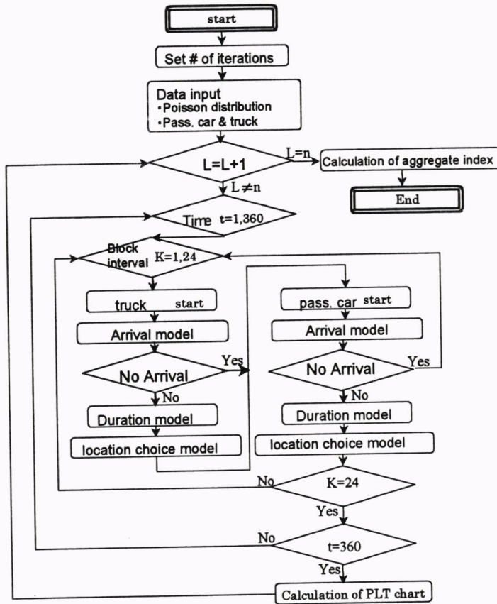
Figure-13 Calculation flow of the simulation system
