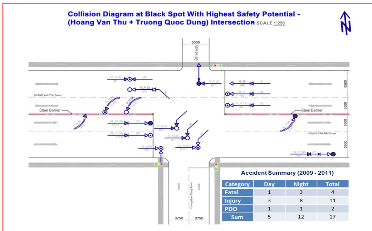
Figure 18. Collision diagram of black spot which has highest SAPO
