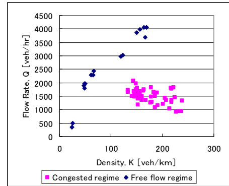
Figure 9. Q - K Plot
