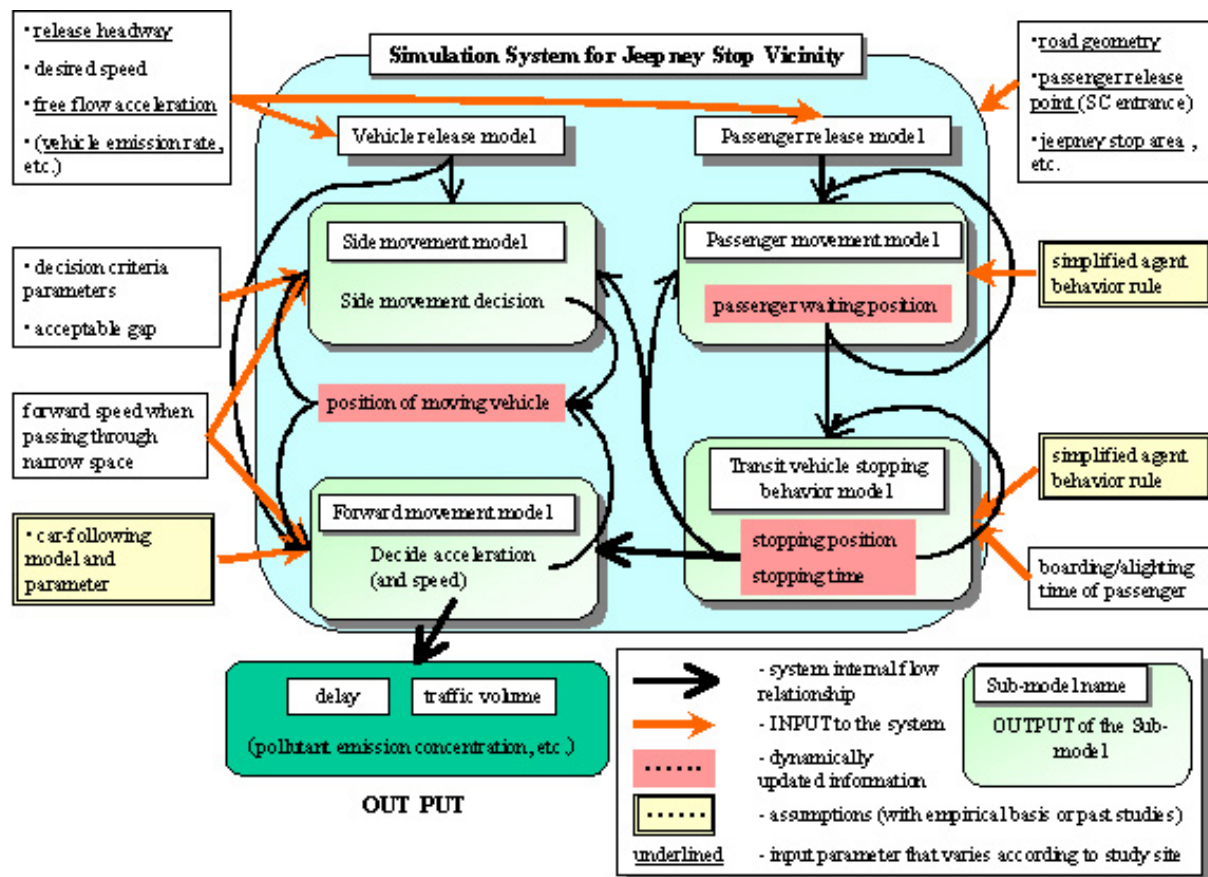
Figure 7. Structure of the simulation model system
