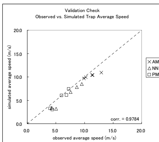
Fig. 10. Observed vs. Simulated Speed
