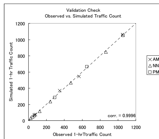
Fig. 11. Observed vs. Simulated Traffic Count
