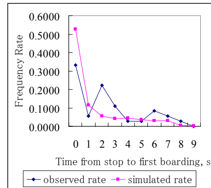
Figure 12. Observed vs. Simulated Time from stop to first boarding
