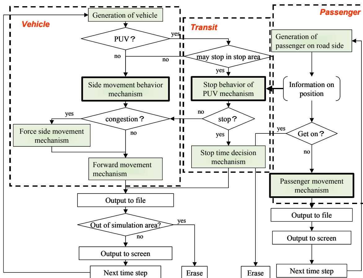
Figure 4. Flow chart of overall simulation logic
