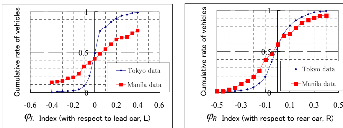
Figures 1 (left) & 2 (right). Cumulative rate of vehicles for varying values of \varphi . (Index \varphi is rate of change of distance headway, a measure of lane changing aggressiveness; Tokyo data from Nakamura et al. , 1992)
